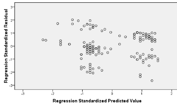
Fig. 2. RSR and the RSP graph
