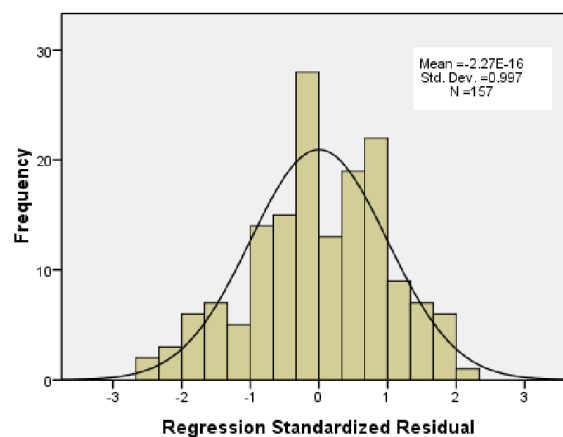
Fig. 1. Frequency and regression standardized residual
